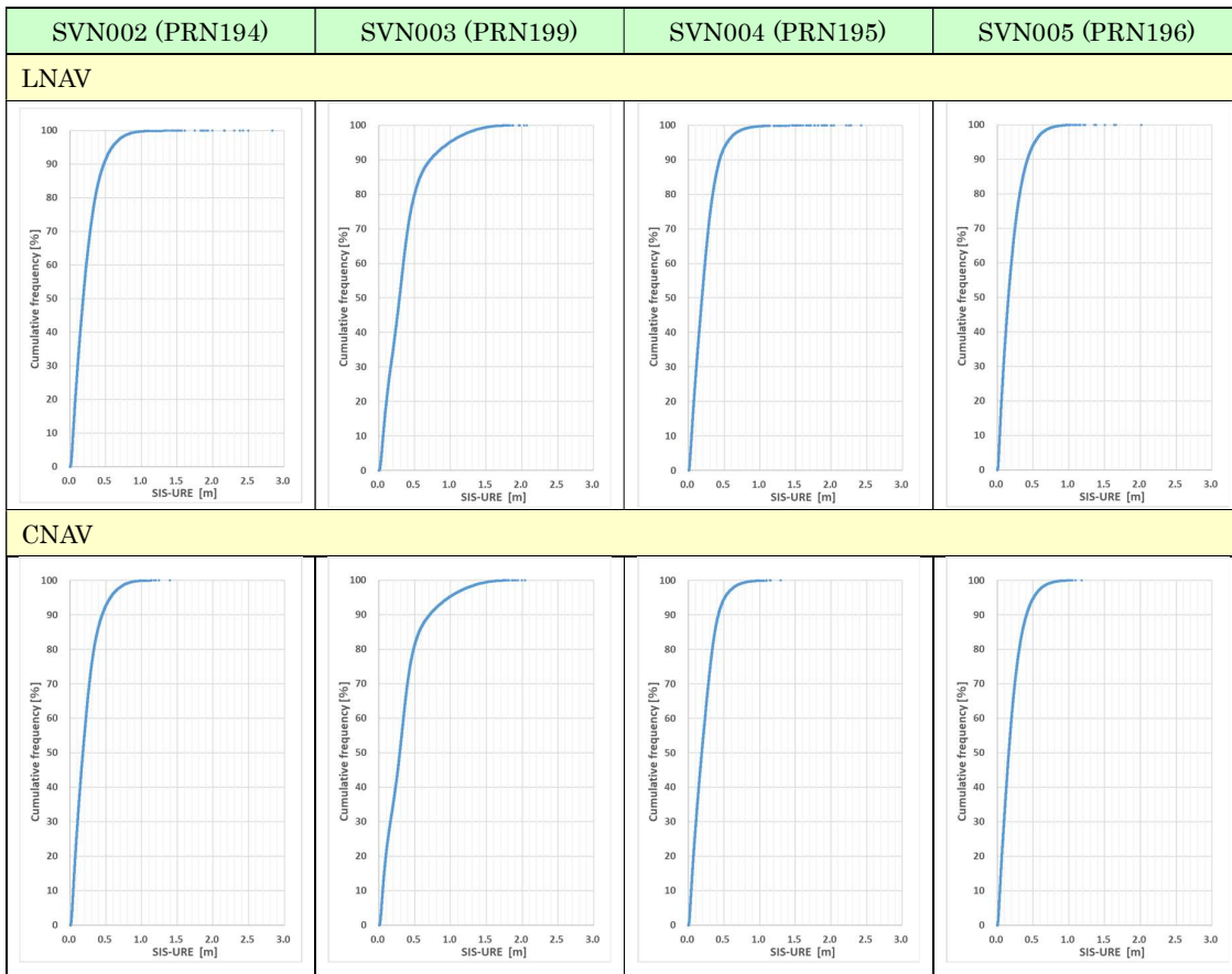
Figure 1 The distribution of SIS Accuracy of the ephemeris
